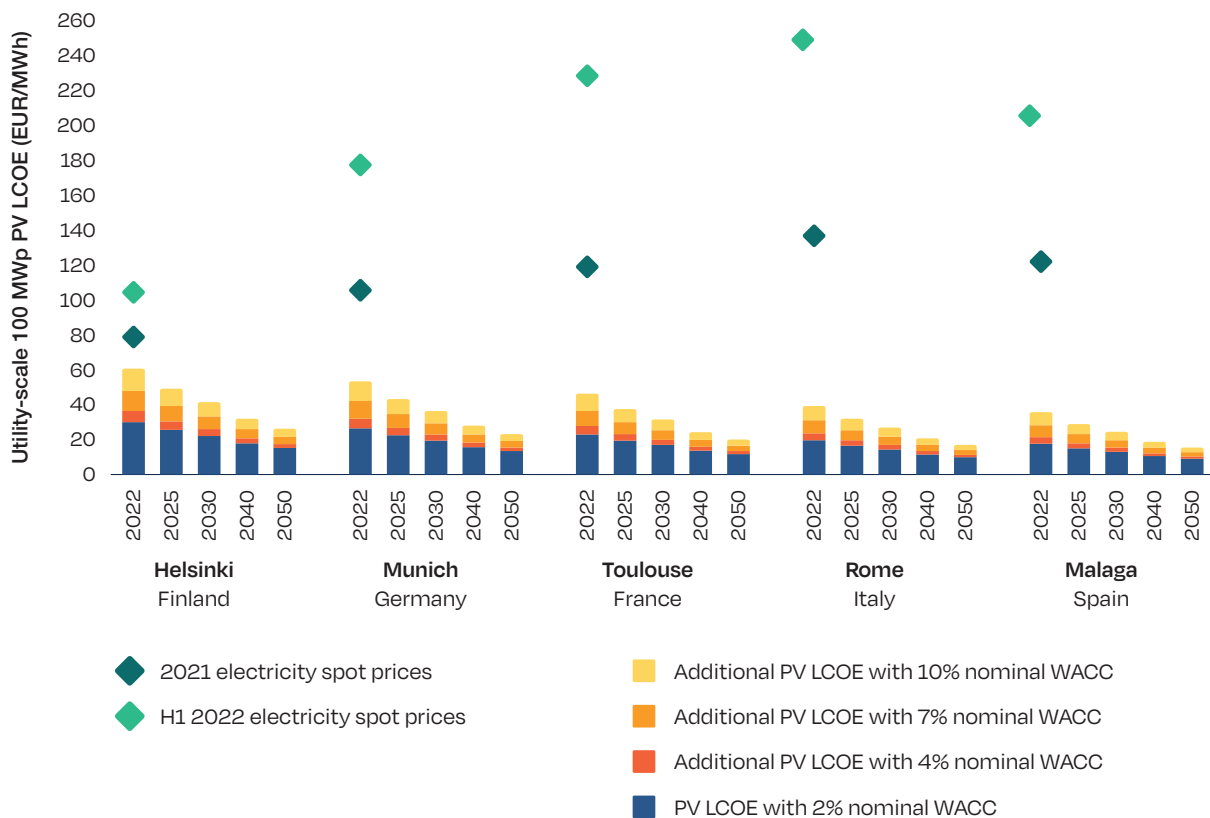
FIGURE 1 PV LEVELISED COST OF ELECTRICITY (LCOE) IN FIVE EU LOCATIONS, 2022-2050
