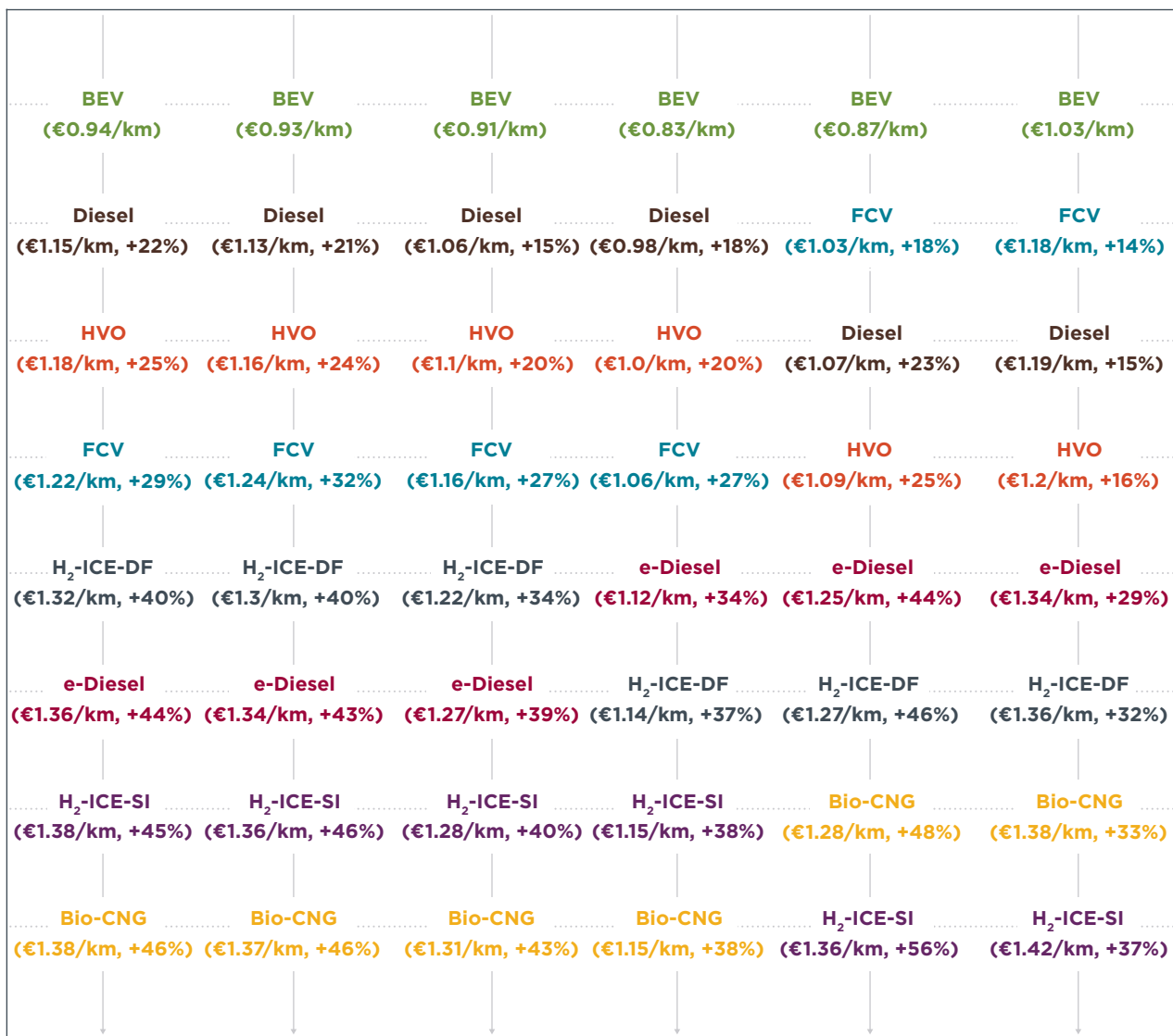
Figure 3. Ranking the TCO performance per different truck classes and powertrain technologies for the model year 2030. The figure shows the TCO of each decarbonization pathway and truck class, and the percentage difference in TCO relative to the least-cost decarbonization pathway.
